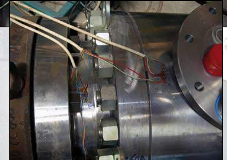
Strain gauge test
